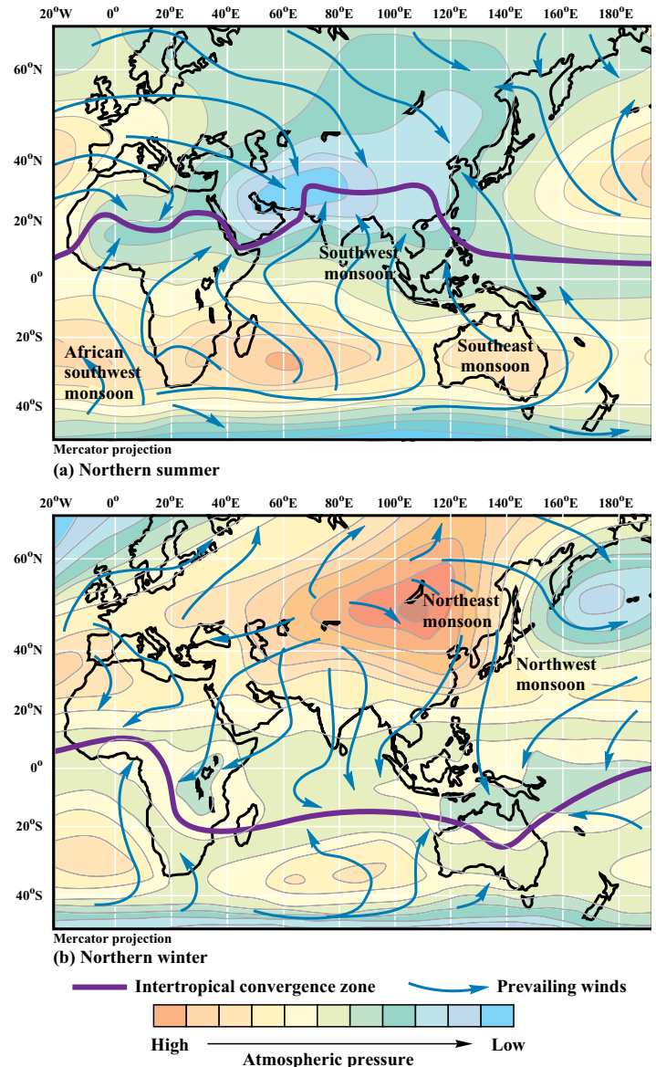
FIGURE 7-12 Indian Ocean monsoon winds. (a) In summer, an intense low-pressure zone forms over Asia as the land is heated by the sun and loses this heat to the atmosphere more quickly than does the ocean. The heated air rises to form the low-pressure zone at a latitude where, if the Earth were covered by ocean, the Hadley and Ferrel cells would intersect and atmospheric pressure would be high. The low-pressure zone causes the atmospheric convection cells to shift to the north and bring warm, wet, southwest monsoon winds to parts of Asia. A similar, but less pronounced effect occurs over North Africa. (b) In winter, the Asian landmass loses heat more quickly than does the ocean, and an intense high-pressure zone is formed by the sinking cold, dry air mass. As this air mass spreads to the south, it shifts the convection cells south, which creates the northeast monsoons and brings dry weather to much of Asia.
