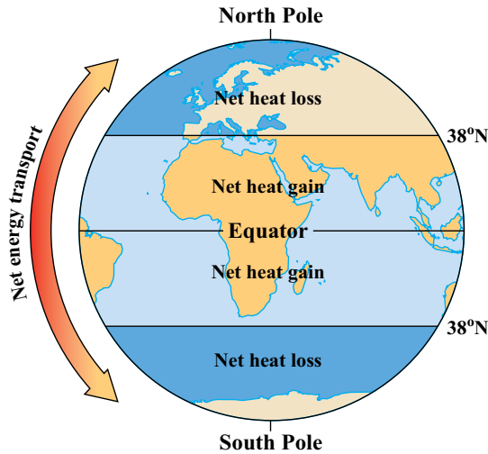
FIGURE 7-7 Variation in radiative heat loss and gain at the Earth's surface with latitude. There is a net gain between the equator and about 35° to 40°, and a net loss at higher latitudes.
