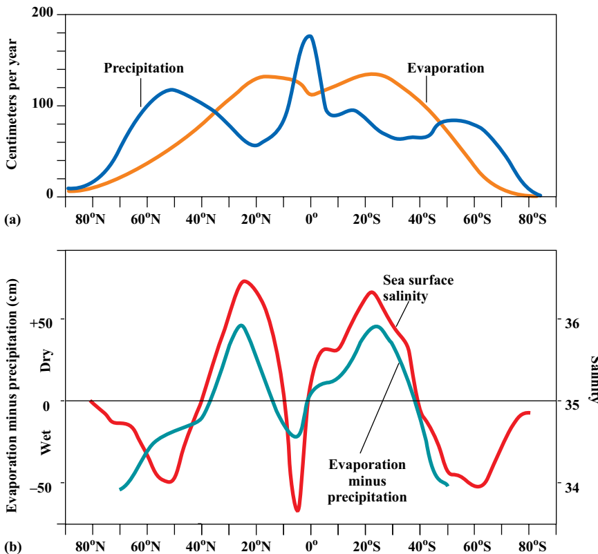
FIGURE 7-15 Precipitation and evaporation as a function of latitude. (a) Precipitation is high at the atmospheric upwelling zones at the equator and at 50° to 60° N and S, somewhat lower in mid latitudes, and very low at high latitudes. Evaporation generally increases from the poles toward the equator, but it is slightly lower at the equator because of the extensive cloud cover. Thus, there is a net excess of evaporation over precipitation in mid latitudes, whereas there is a net excess of precipitation within a few degrees north and south of the equator and at latitudes above approximately 40° in both hemispheres. (b) The salinity of surface ocean waters varies according to the difference between evaporation and precipitation. It is high where evaporation exceeds precipitation, and low where precipitation exceeds evaporation.
