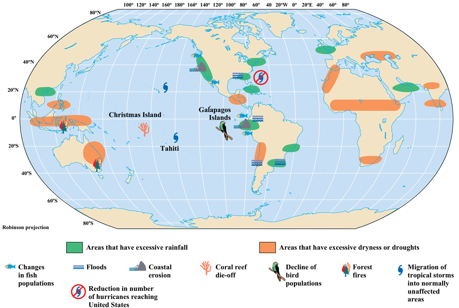
FIGURE 7-19 Strong El Niño events have worldwide effects that, in different areas, include droughts, excessive rainfall and floods, coastal erosion, tropical storms in areas where they do not normally occur, and various changes in terrestrial and marine ecosystems, some of which can be disastrous.
