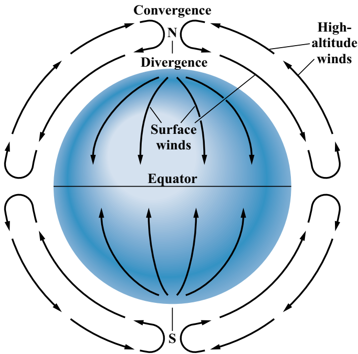
FIGURE 7-8 Atmospheric convection cells and winds on a hypothetical water-covered, nonrotating Earth.
