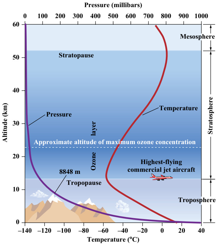
FIGURE 7-1 Structure of the atmosphere. The atmospheric circulation that determines the Earth’s climate and weather takes place within the troposphere. Movements of gases between the troposphere and the stratosphere are limited and slow. Ozone is present throughout the stratosphere, but its concentration peaks at an altitude of about 22 km.
