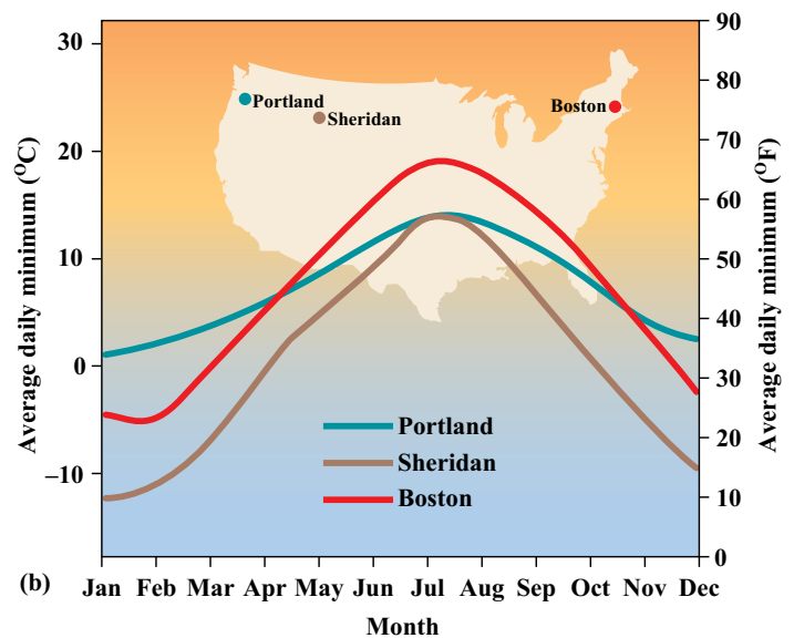
FIGURE 7-24 Annual variation in monthly average air temperature for Portland, Oregon; Sheridan, Wyoming; and Boston, Massachusetts. (a) Daily high temperatures. (b) Daily low temperatures. These cities are at approximately the same latitude; however, their climates are very different. Portland has a maritime climate with a small annual temperature range; Sheridan has a continental climate with a large annual temperature range; and Boston has a more continental climate than would be expected from its coastal location, because the climatic winds there blow from the continent toward the ocean.
