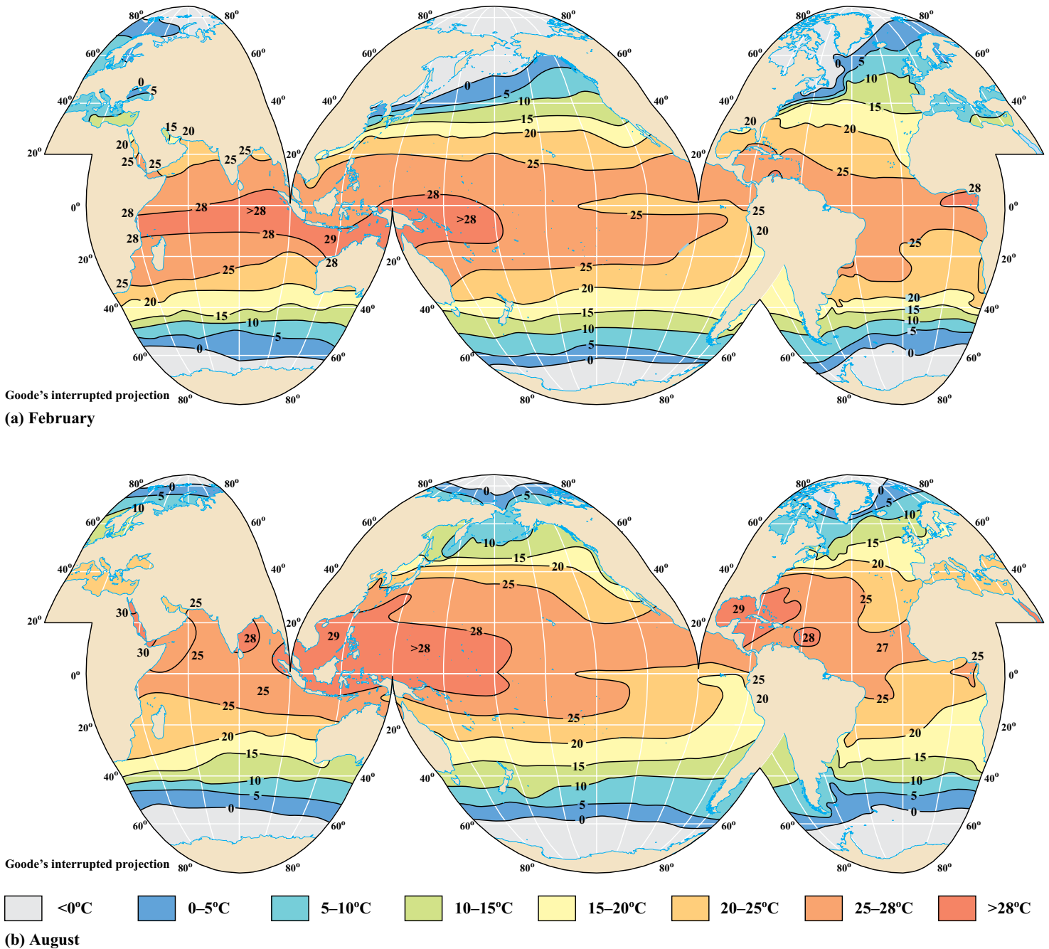
FIGURE 7-13 Average surface water temperatures in the world oceans in (a) February and (b) August.
