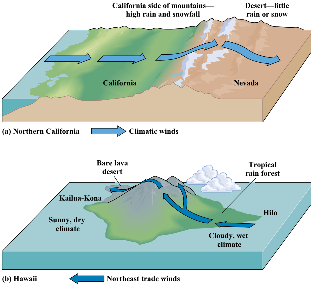
FIGURE 7-32 The mountain or island effect occurs where a moving mass of moist air, usually from over the ocean, encounters a mountain or mountainous island, rises, cools adiabatically, and loses water as rain or snow. Once over the mountains, the air mass descends, warms, and can hold more moisture. As a result, rain and snowfall stop. (a) The Sierra Nevada mountains of California intercept moist air moving inland from the ocean. Rain and snowfall are abundant on the California side of the mountains, but the Nevada side is a desert. (b) On the Hilo side of Hawaii, trade winds blowing from the northeast produce clouds, plentiful rainfall, and tropical rain forests, but the opposite side of the island, near Kailua-Kona, is sunny and has low rainfall.
