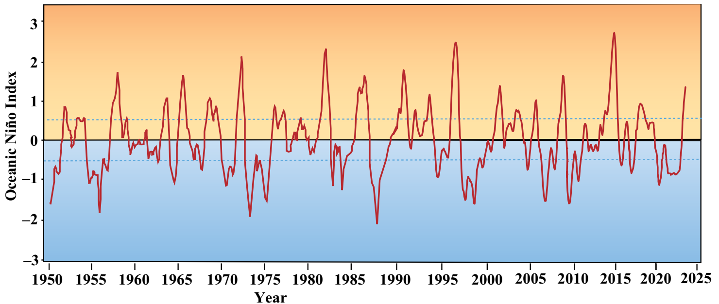
Figure 7-20. The NOAA Oceanic Niño Index since 1950. The index is based on the average surface water temperature in a defined region of the central tropical Pacific Ocean. El Niño (when the index rises above 0.5) and La Niña (when the index falls below -0.5) have occurred regularly about every 3-5 years.
