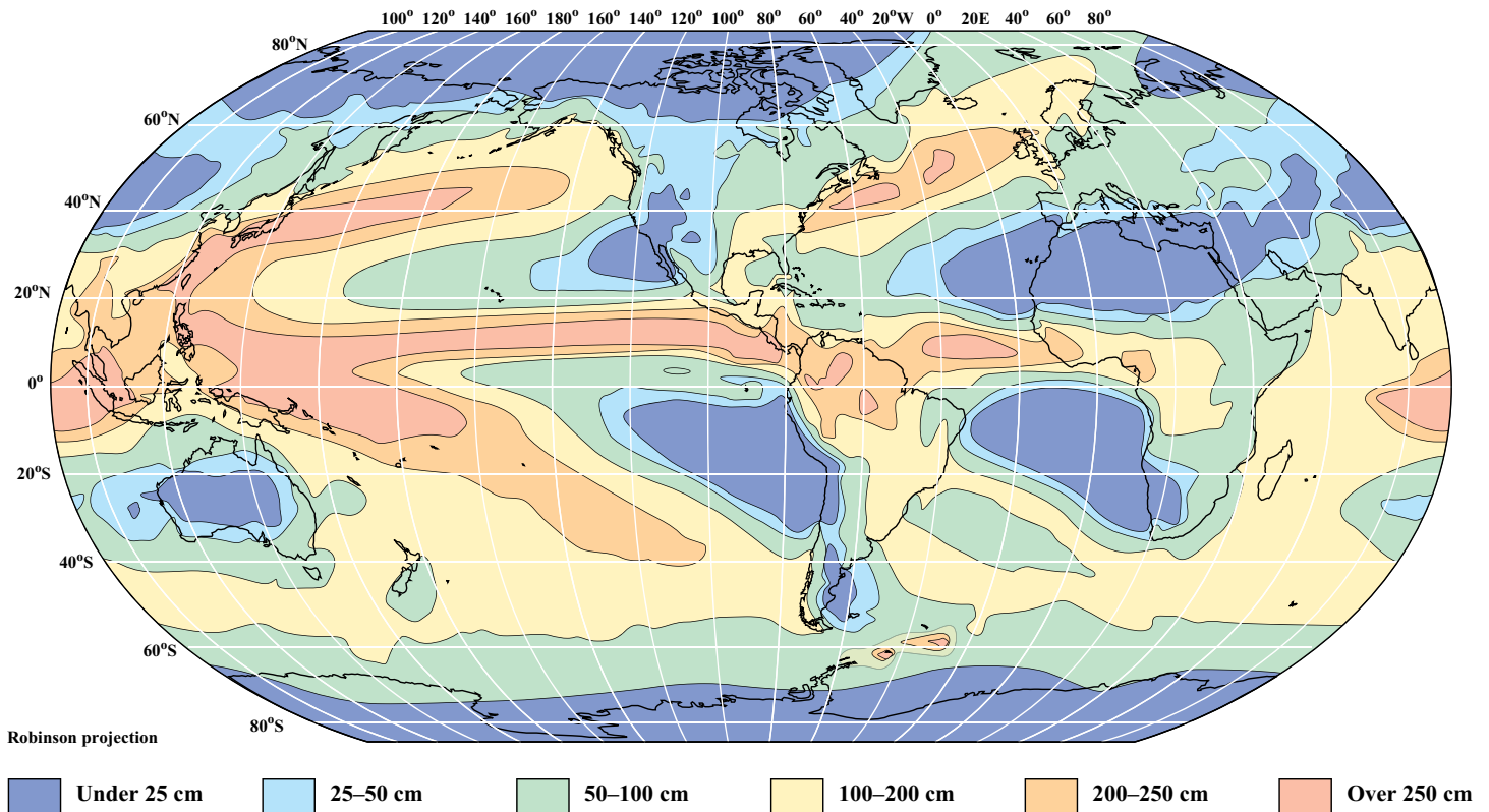
FIGURE 7-16 Distribution of mean annual atmospheric precipitation. Precipitation is high in the tropical atmospheric upwelling zone at the equator, generally low at mid latitudes in the atmospheric downwelling zones between the Hadley and Ferrel cells, higher in the atmospheric upwelling zones between the Ferrel and polar cells, and low again in the polar atmospheric downwelling zones. This pattern is more evident in the Southern Hemisphere because it is less modified by the presence of landmasses than it is in the Northern Hemisphere.
