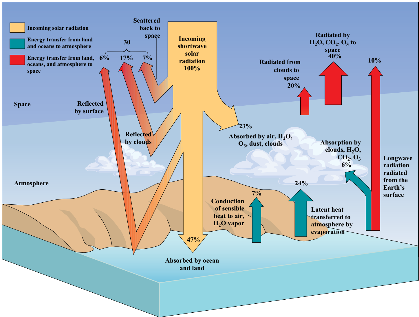
FIGURE 7-5 The Earth's heat budget. Solar radiation, which is concentrated in the visible light wavelengths, is reflected, scattered, and absorbed by the gases and clouds of the atmosphere and by the ocean and land surface. All of the absorbed energy is radiated back to space, primarily as infrared radiation. The diagram shows the estimated percentages of the incoming solar radiation that are absorbed, reflected, and reradiated to space by the various components of the Earth–ocean–atmosphere system. Each of these may change in an unpredictable way as the greenhouse effect is enhanced by anthropogenic inputs to the atmosphere (CC9, CC10, CC11).
