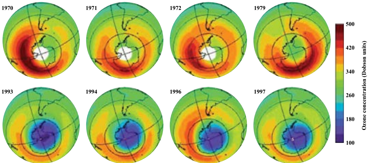
Average atmospheric ozone concentrations for October of each year shown
