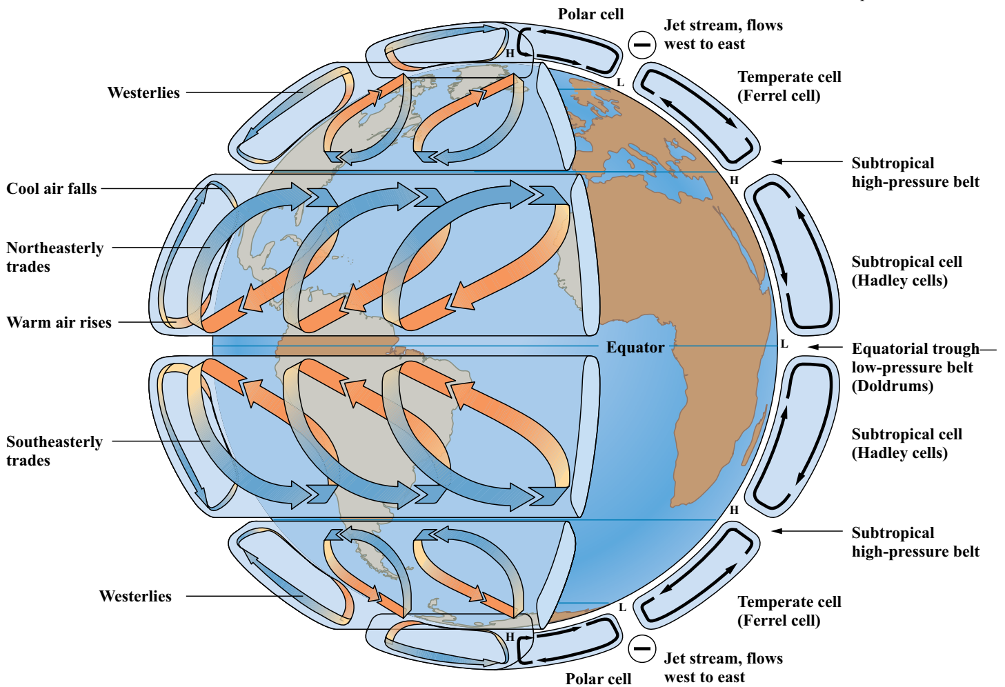
FIGURE 7-9 Atmospheric convection cells and winds on a hypothetical water-covered, rotating Earth are arranged in latitudinal bands. There are three cells in each hemisphere. Upwelling occurs at the equator and the polar fronts, and downwelling at the poles and in mid latitudes. Note how the Coriolis effect deflects air masses: air masses moving away from the equator are deflected to the east, and air masses moving toward the equator are deflected to the west. Atmospheric convection cells are arranged in this general pattern on the Earth, but they are modified substantially by the influence of the land masses.
