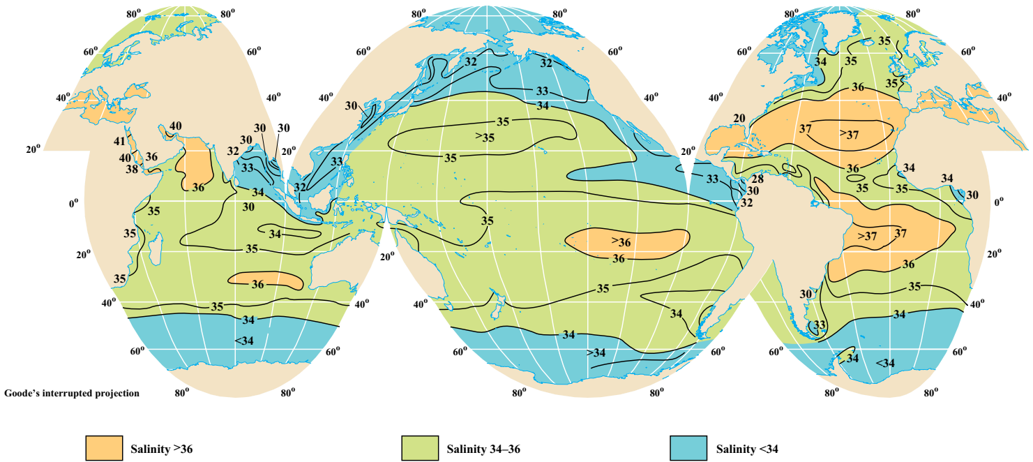
FIGURE 7-14 Surface water salinity in the world oceans.
