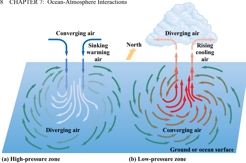
FIGURE 7-25 Geostrophic winds and zones of high and low pressure. (a) Cold, dense air sinks, creating a high-pressure zone in the lower atmosphere. The sinking air warms and flows out from the high-pressure zone. As the air flows outward, it is deflected by the Coriolis effect and forms geostrophic winds that flow clockwise around the high-pressure zone (counterclockwise in the Southern Hemisphere). (b) Warm, moist air rises, creating a low-pressure zone in the lower atmosphere. The rising air cools, and water vapor condenses, causing precipitation. The warm rising air at the center of the low-pressure zone is replaced by air drawn toward the low from across the Earth's surface. As the air flows inward, it is deflected by the Coriolis effect and forms geostrophic winds that flow counterclockwise around the low-pressure zone (clockwise in the Southern Hemisphere).
