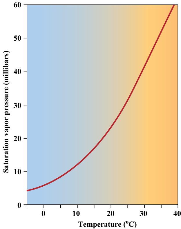
FIGURE 7-3 Variation of the water vapor saturation pressure with temperature. Air can hold less water vapor at lower temperatures. This is the reason that water condenses into rain as warm, moist air rises and cools adiabatically.
