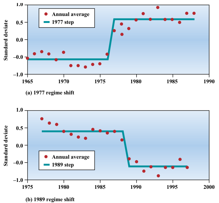
FIGURE 7-21 Variations in a composite index of environmental variables related to climate in the North Pacific Ocean. Time series were examined for 100 variables—31 climatic and 69 biological—although data were not available for all variables throughout the analysis period. (a) A regime shift occurred in the winter of 1976–1977, as shown by the step change in this function, which includes time series for 91 variables. (b) A regime shift also occurred in 1989, as shown by the step decrease in an index that includes time series for 94 variables. However, this second shift did not return the system to the same state as before 1977.
