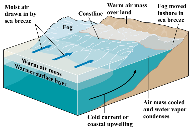
FIGURE 7-31 Coastal fog develops when moist air is drawn inland by a sea breeze or climatic winds and passes over a cold nearshore water mass. The cold nearshore water can be the result of cold-water currents or, more often, of coastal upwelling that brings cold, deep water to the surface.
