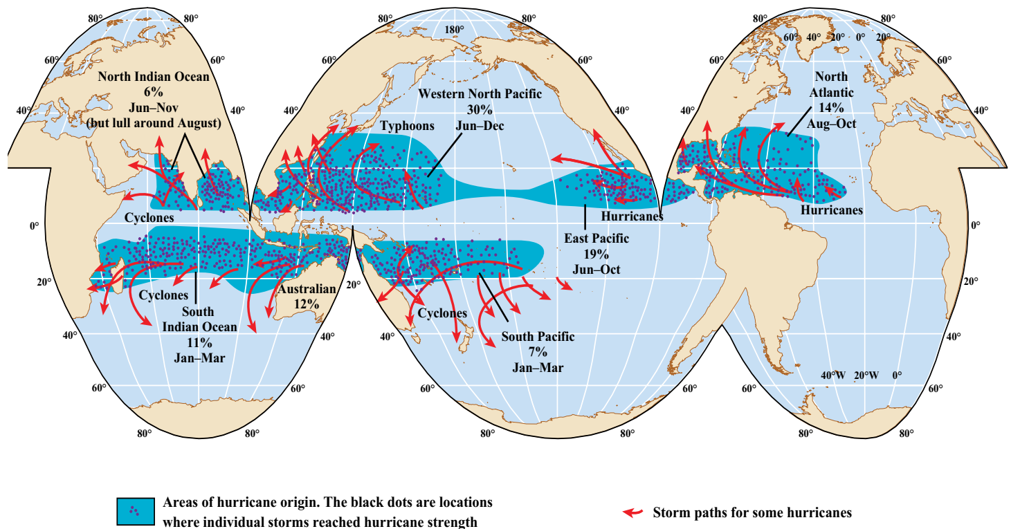
FIGURE 7-28 Hurricanes develop where the surface ocean water temperature is greater than 26°C, except in the equatorial region between 5°N and 5°S, where the Coriolis effect is too weak to generate these storms. Surface waters are too cold for strong tropical storm formation in the eastern Atlantic Ocean and below the equator in the eastern Pacific Ocean. Once formed, hurricanes travel generally east to west, curving toward higher latitudes as they are steered by the Coriolis effect and by other weather systems. Hurricanes are most frequent in the western North Pacific Ocean, where they are called “typhoons” or “baguios.”
