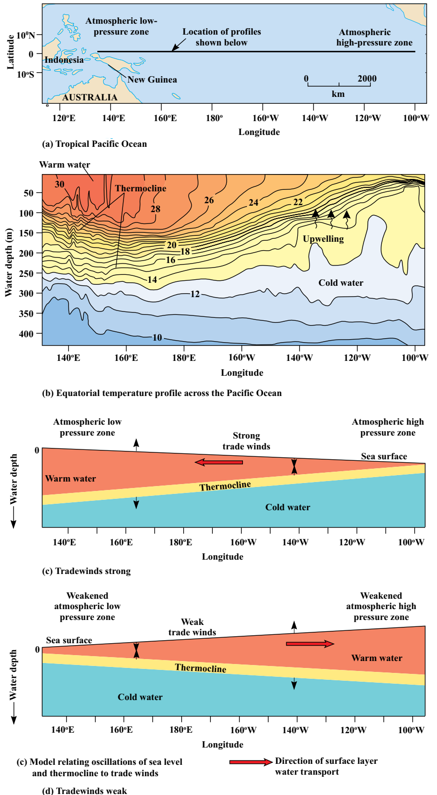
FIGURE 7-18 One possible model for the development of El Niño. (a) The area of the Pacific Ocean where El Niño develops. (b) When trade winds are strong, warm surface water is pushed westward and piles up on the western boundary of the Pacific Ocean near Indonesia. The surface layer is thinned near Peru, and upwelling occurs. (c,d) The vertically exaggerated cross sections are a simplified depiction of the interaction of trade winds with sea-level and thermocline depth in the two extreme modes of ENSO. The cross section in part (c) shows the effect of strong trade winds on the sea surface and surface water layer. This is the normal, or in extreme cases, the La Niña situation. When the trade winds diminish, surface layer water is transported eastward toward Peru, resulting in the El Niño situation shown in part (d). In an El Niño, the surface layer is thickened near Peru, and upwelling ceases.
