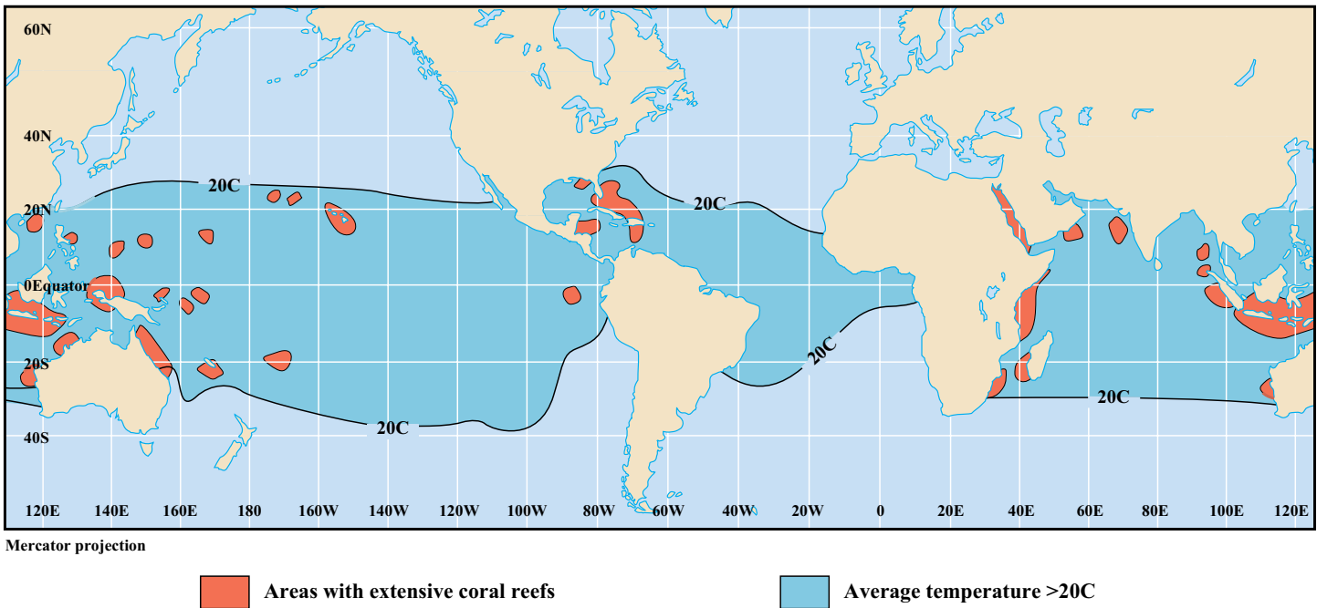
FIGURE 15-2 The area of the oceans with average sea surface temperatures above 20°C extends to about 30° north and south of the equator in the Pacific and Indian oceans, and somewhat less in the Atlantic Ocean. The temperature never falls below 18°C in most of this area. Hermatypic corals grow only in these areas and only where other environmental conditions are suitable within these areas. Although many small tropical islands have extensive coral reefs, they are too small to show in this figure.
