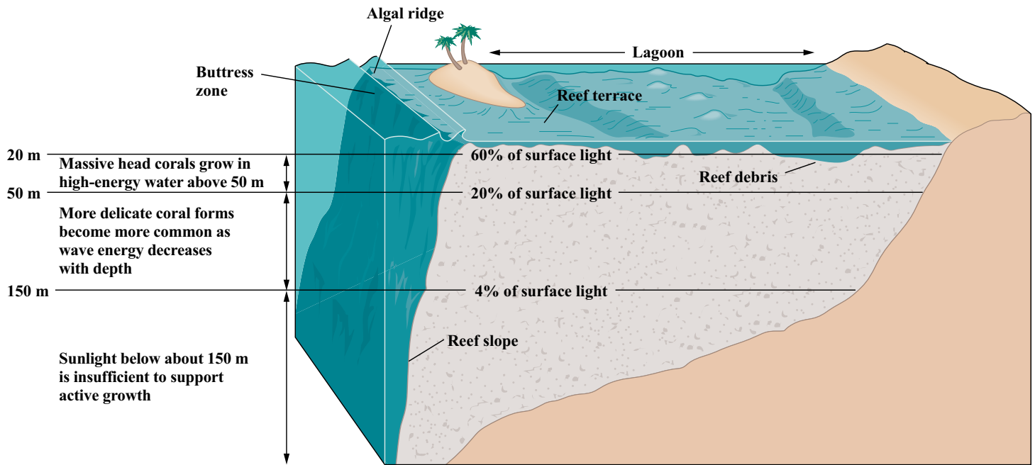
FIGURE 15-3 Structure of a typical coral reef
