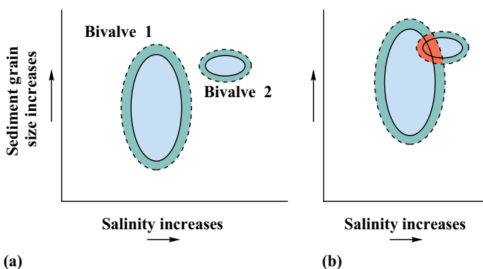
FIGURE 15-1 Ecological niches can be defined in several ways and by many parameters. These diagrams illustrate the concepts using just two such parameters: salinity and sediment grain size. (a) The fundamental niches of two bivalves are defined by the range of values of the two parameters defined by the blue areas. The survival niches are defined by a wider range of environmental conditions and include both the blue and green areas within each dotted line. Because the niches of these two species do not overlap, they would not occur in the same environment. (b) If the niches of the two species overlap, as they do in the red area, they may both occur in environments within this range of the two parameters, but they may also compete such that one species may be excluded from this part of its niche.
