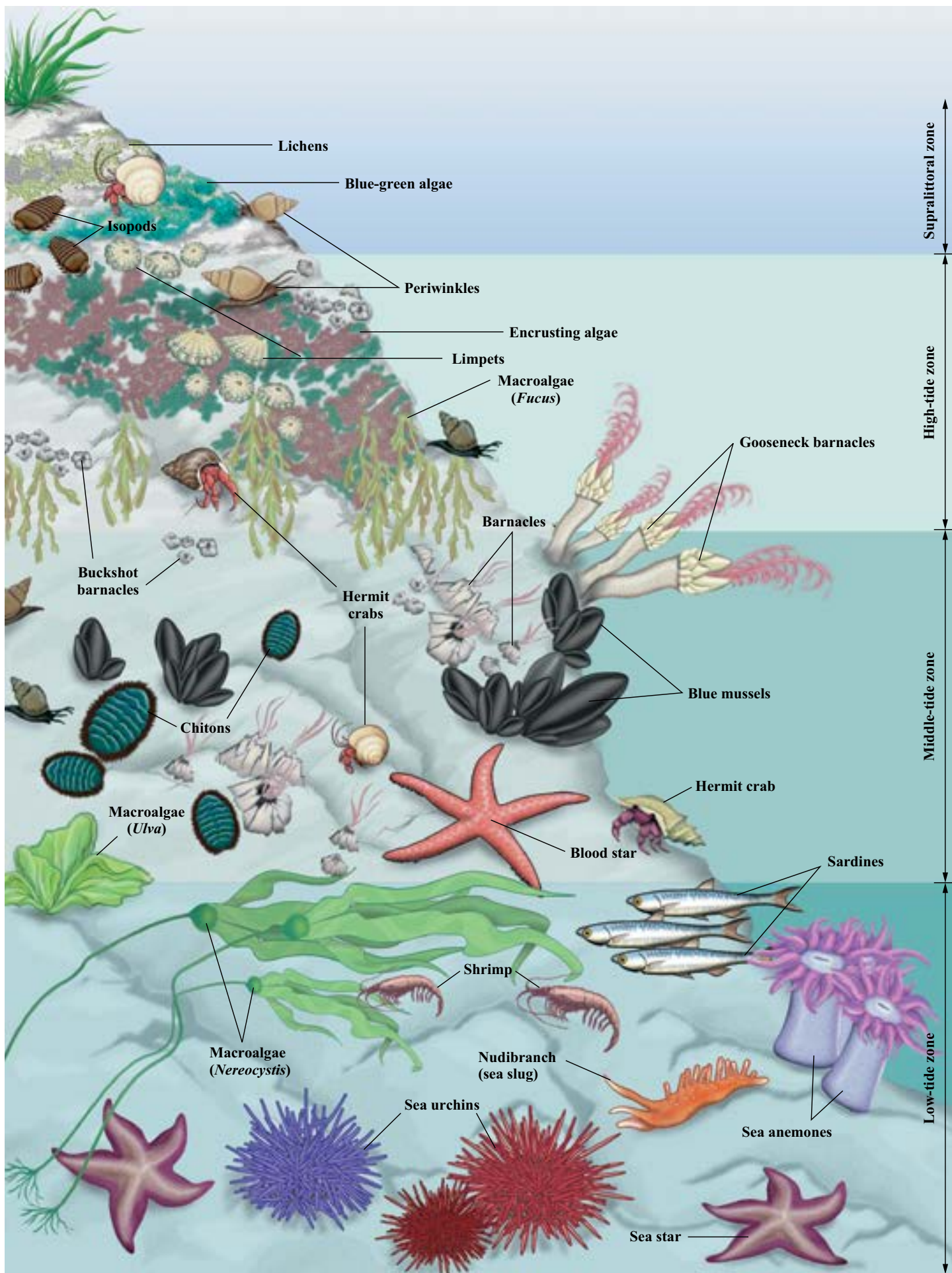
FIGURE 15-11 The rocky intertidal shoreline can be separated into four zones based on length of time exposed to the atmosphere. Many species have ecological niches that restrict them to only one of these zones, although closely related species may occupy different zones. The flora and fauna in this figure are typical of a mid-latitude, cold-water, rocky shoreline. Generally, many more species occur in each zone than are shown here. Competition between species often determines the vertical limits of a particular species' distribution within the zone that it occupies.
